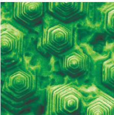
SEM image of AlGaIn epilayer X L Wang et al 2007 J. Phys.: Condens. Matter 19 176005.
