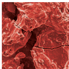
Arrested cracks in porous SiC quenched from 1200°C to 20°C S Ding et al 2007 J. Phys. D: Appl. Phys. 40 2138–2142.
