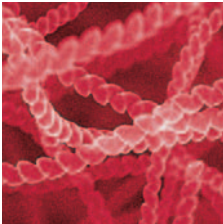
An SEM image of carbon nanocoils synthesized on copper micro-tips at 600 °C W Y Sung et al 2007 Nanotechnology 18 245603.
